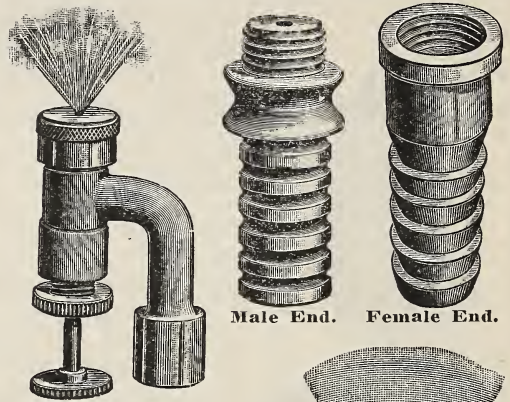
Vermorel Nozzle.
